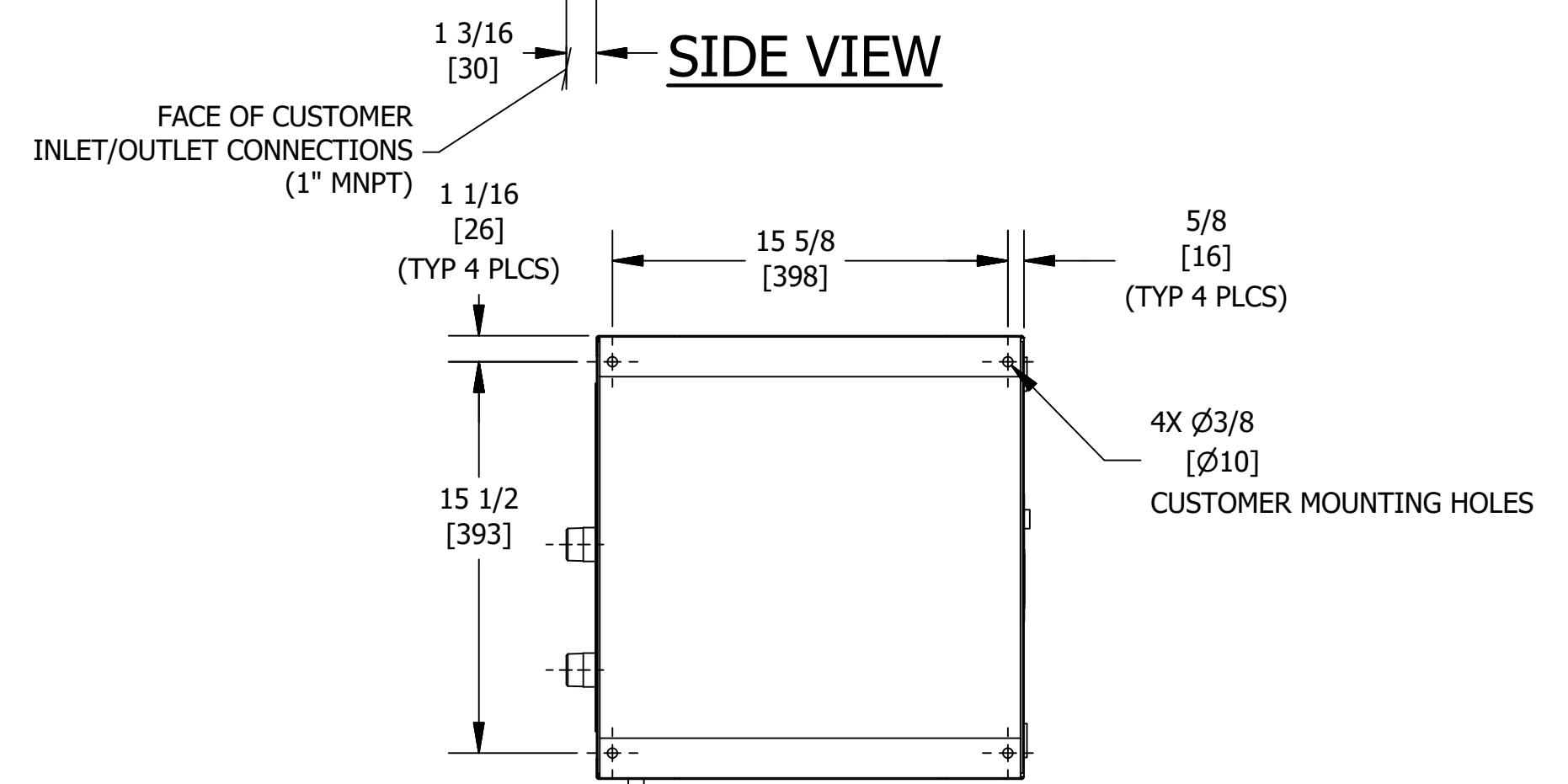
FOOT PRINT
