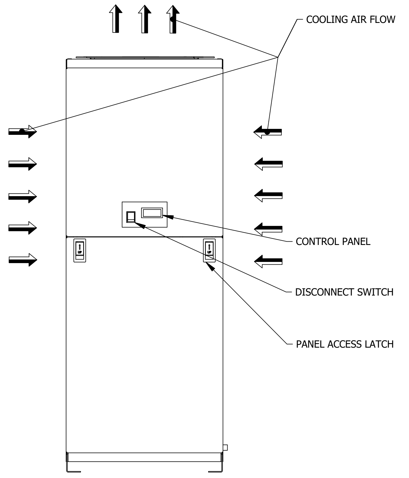
FRONT VIEW
