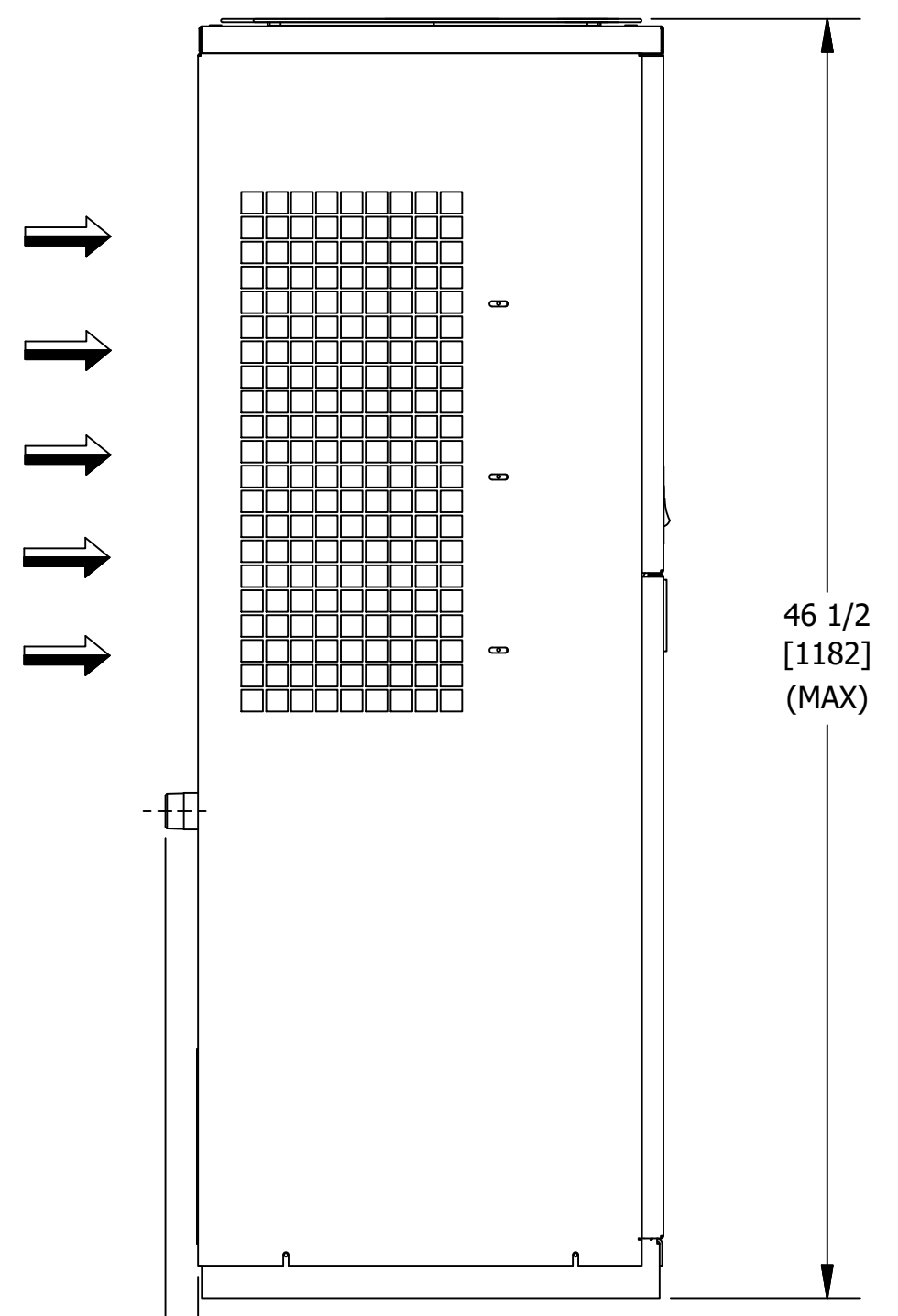
SIDE VIEW
